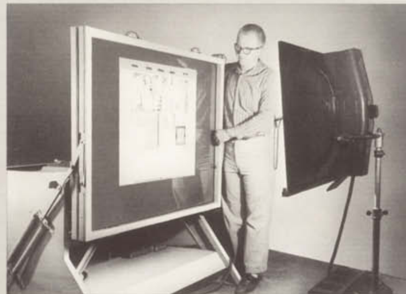
Carbon arc light exposing an offset litho plate in vacuum frame.
